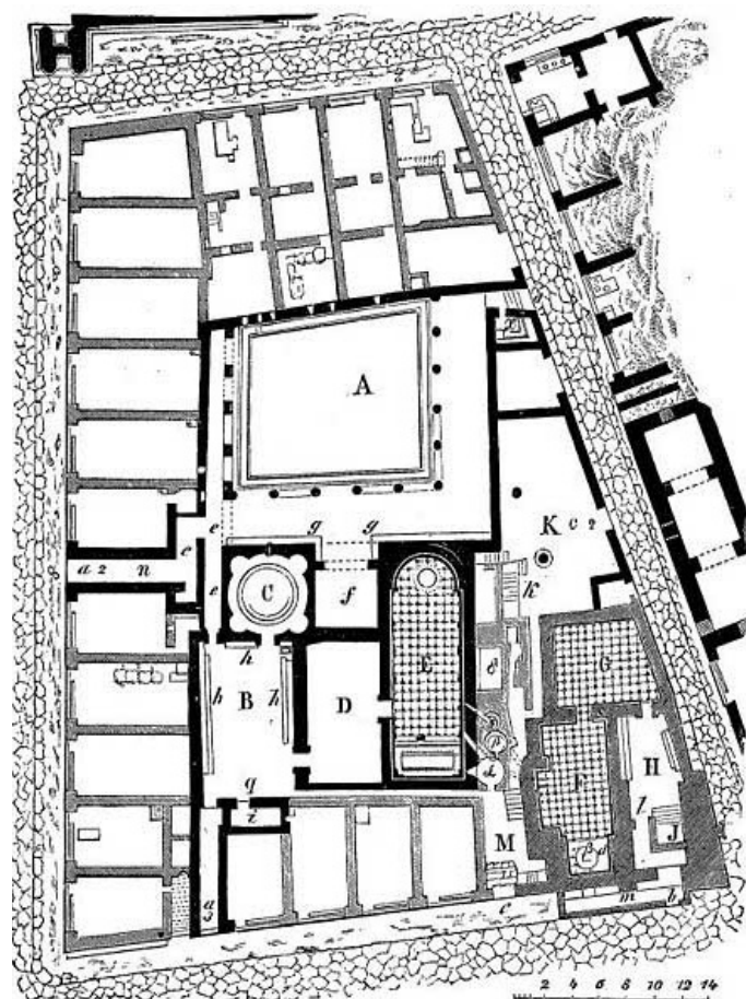
Plan of the Old Baths at Pompeii. (Overbeck.)
